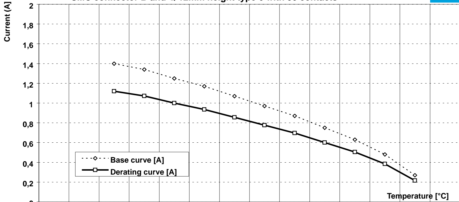
DERATING CURVE (Current carrying capacity acc. IEC 60512-5-2 Test 5b) SMC connector B and Q 12mm height type 6 with 50 contacts
